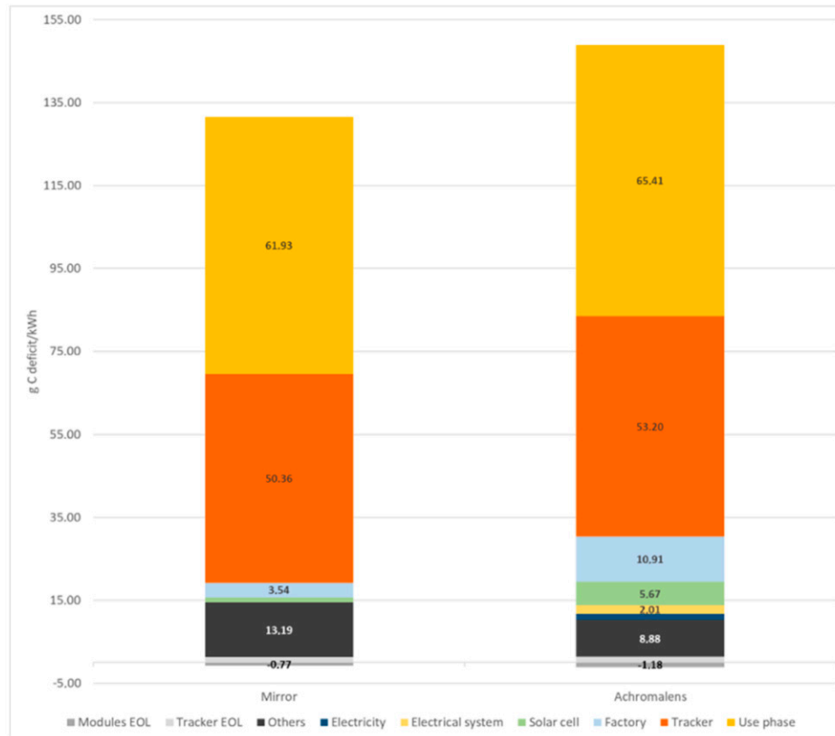
Figure 4. Land-use impact distribution for the mirror and the achromatic lens systems. The mirror system impact is 131.3 g C deficit. However, the achromatic system impact is 147.8 g C deficit. All processes contributing to more than 5% are detailed. Less significant processes are gathered in the “Others” category. Small benefits from recycling metals (gold in particular) explain the negative impact from the modules’ end-of-life.
